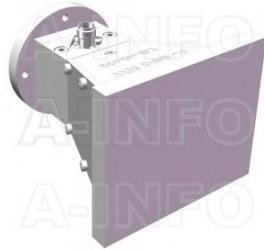
LB-40400-KFSPO Broadband Horn Antenna 4-40GHz 13dB Gain 2.92mm Female
