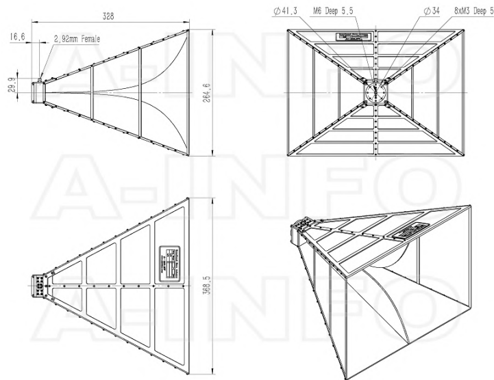
2.92mm-Female Output (P/N: LB-5300-KF)
