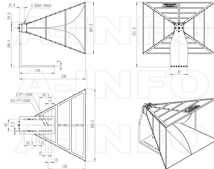
2.92mm-Female Output with L Type Mounting Bracket (Option, P/N: LB-5400-L)
